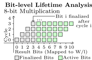
Fig. 15. Bit-level lifetime analysis
