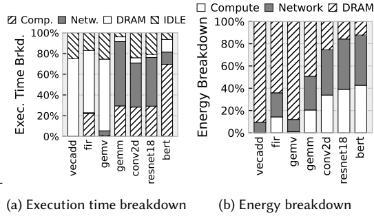
Fig. 18. Categorized breakdown of each workload.
