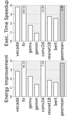
Fig. 16. Comparing PIMSAB with NVIDIA A100
