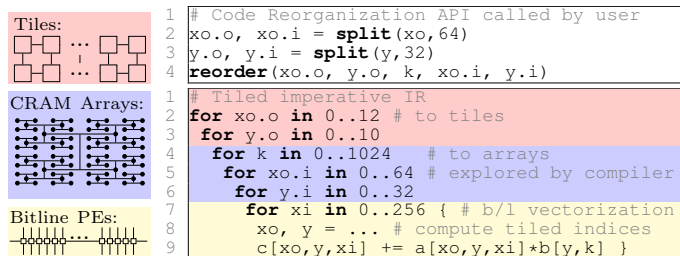
Fig. 13. Reorganize the loops for parallelism distribution.
