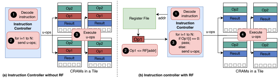
Fig. 11. Flow for constant operations
