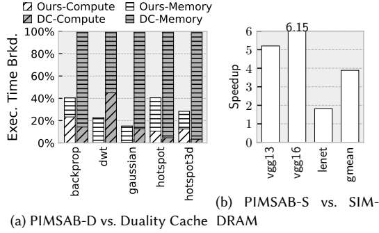
Fig. 17. Appropriately provisioned PIMSAB compared with prior in-SRAM and in-DRAM systems.
