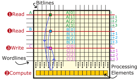
Fig. 1. Basics of bit-serial Processing-In-Memory
