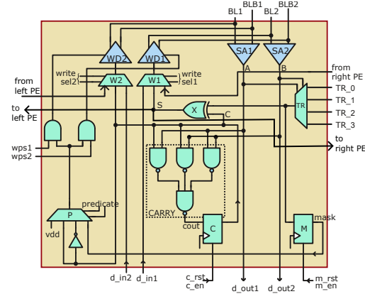
Fig. 5. Processing element used in CRAMs
