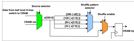
Fig. 9. Shuffle Logic at input of each CRAM in PIMSAB
