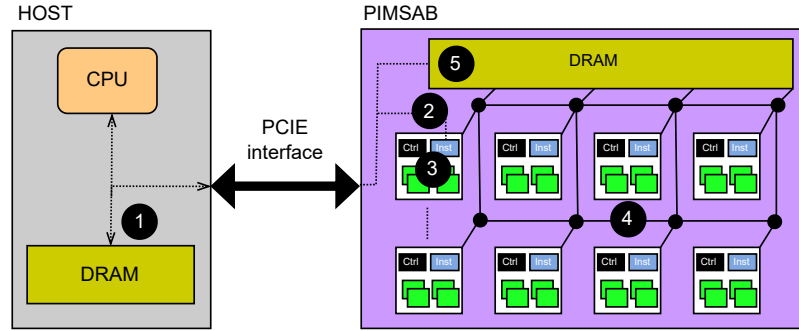
Fig. 4. System Level Architecture
