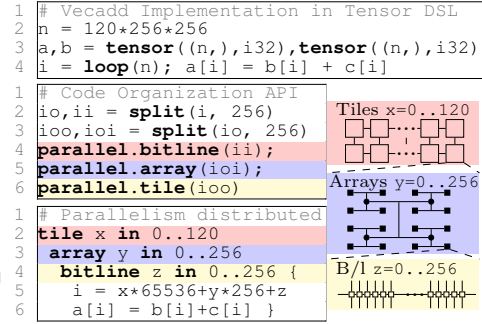
Fig. 2. Programming PIMSAB in tensor DSL.
